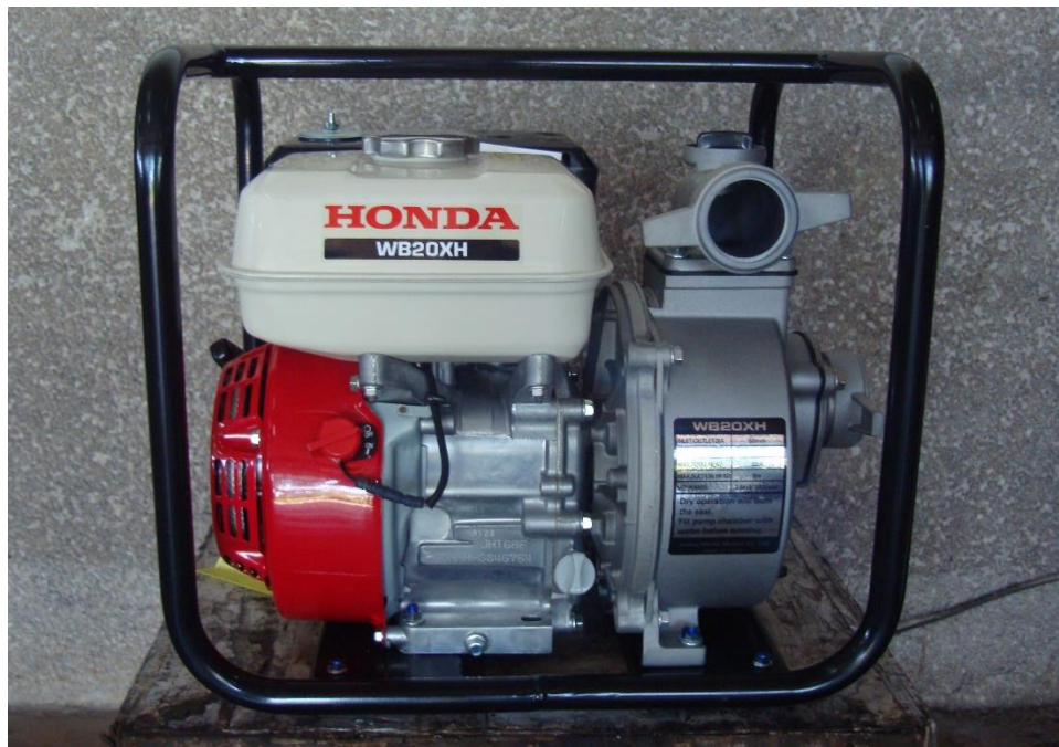
Figure 2. HONDA WB20XH Self-priming Centrifugal Pumpset
