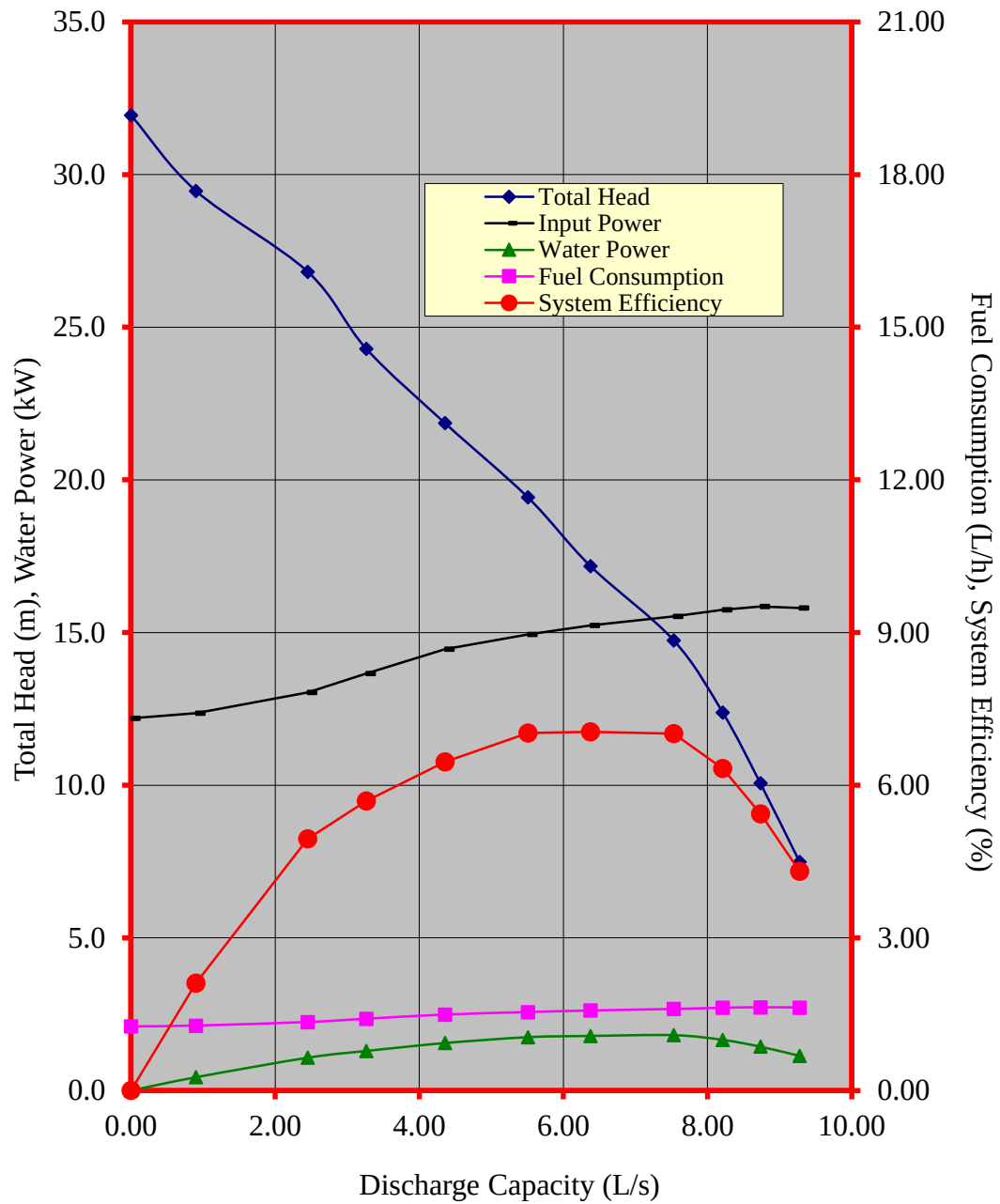
Figure 3. Performance characteristic curves of the HONDA WB20XH self-priming centrifugal pumpset
